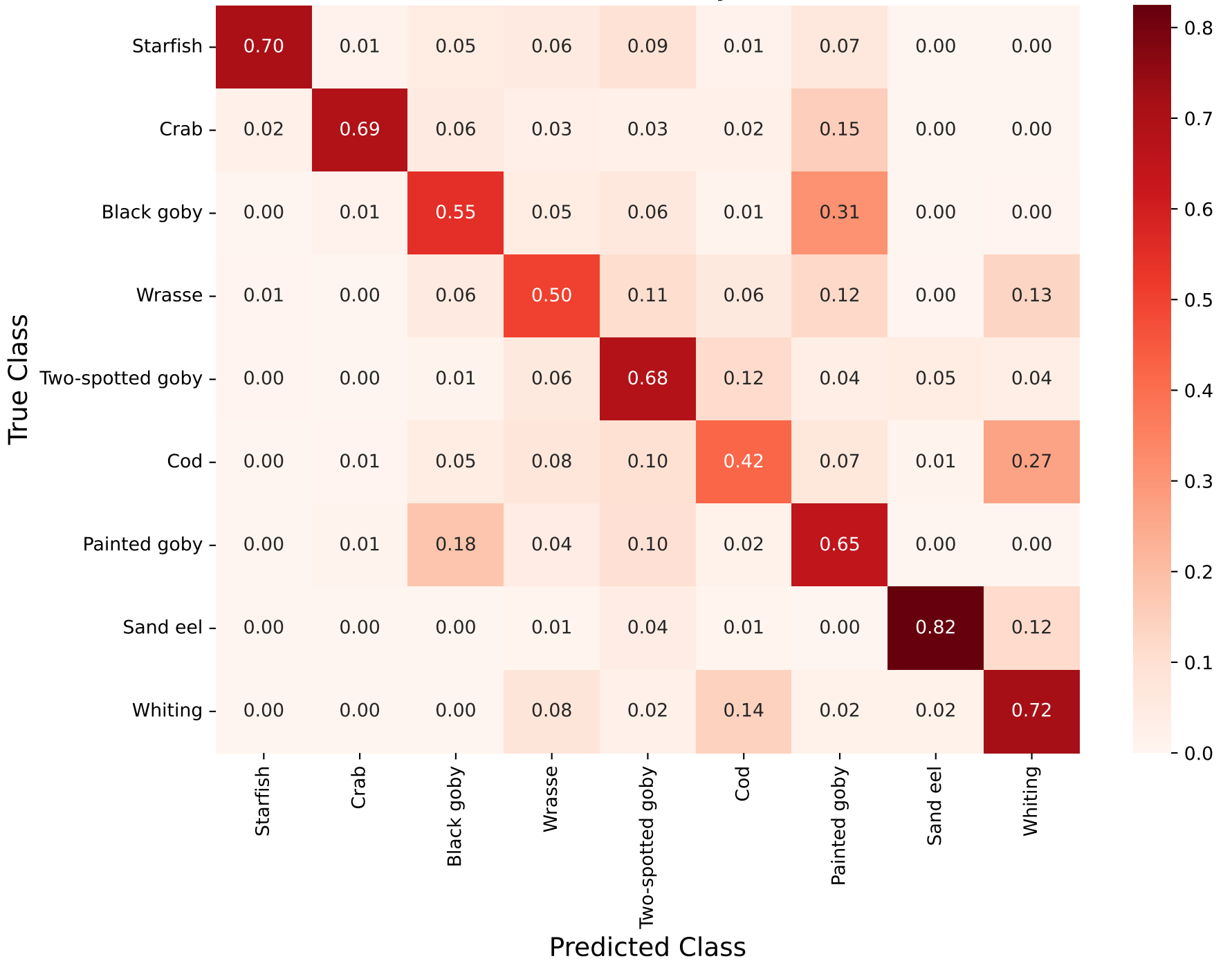
Heat map (row normalised) of DINOv2 embeddings normalised median analysis
