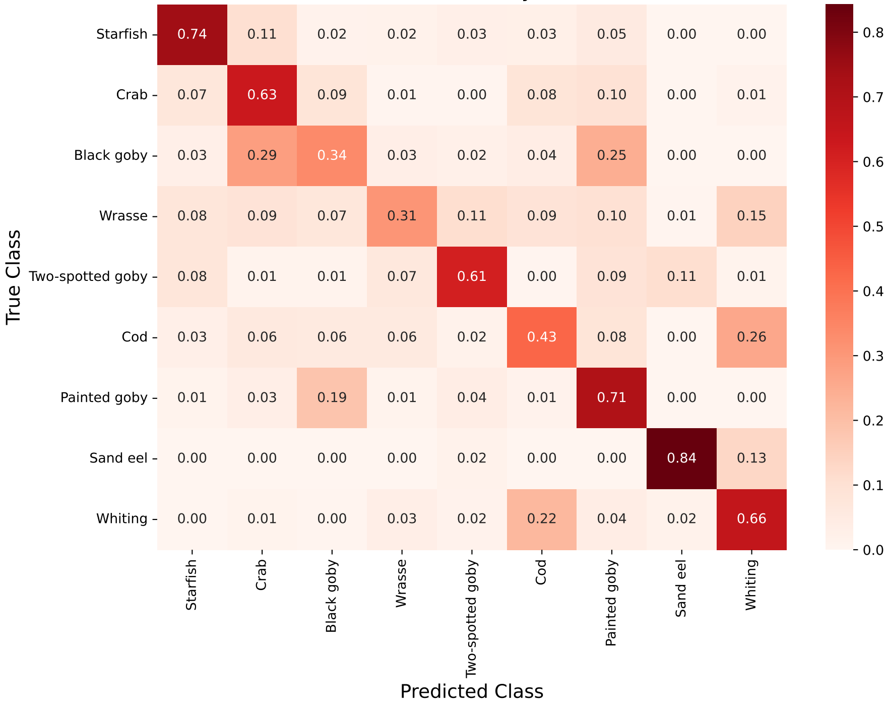
Heat map (row normalised) of resnet embeddings median analysis
