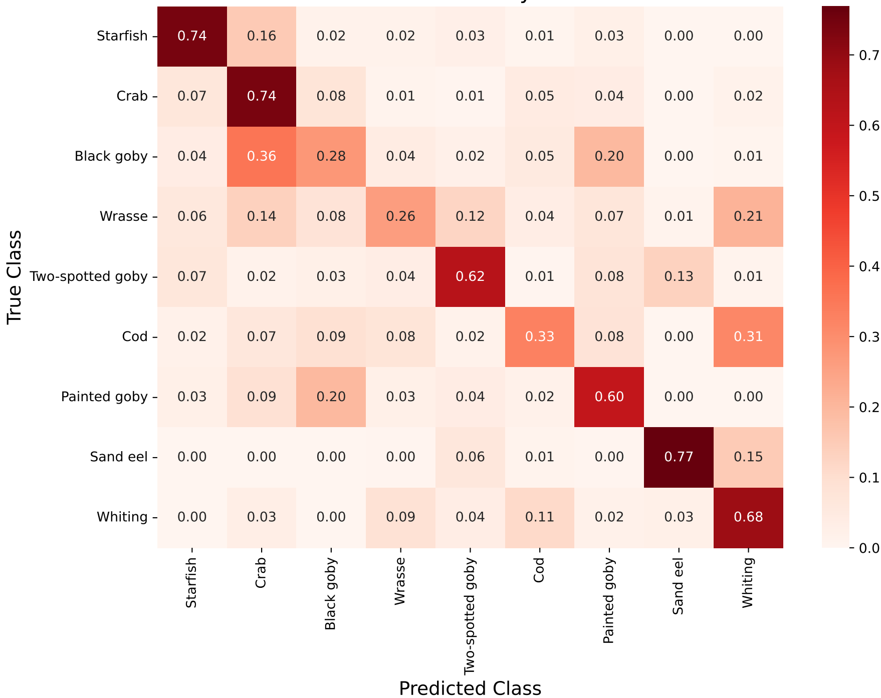
Heat map (row normalised) of resnet embeddings gray normalised median analysis
