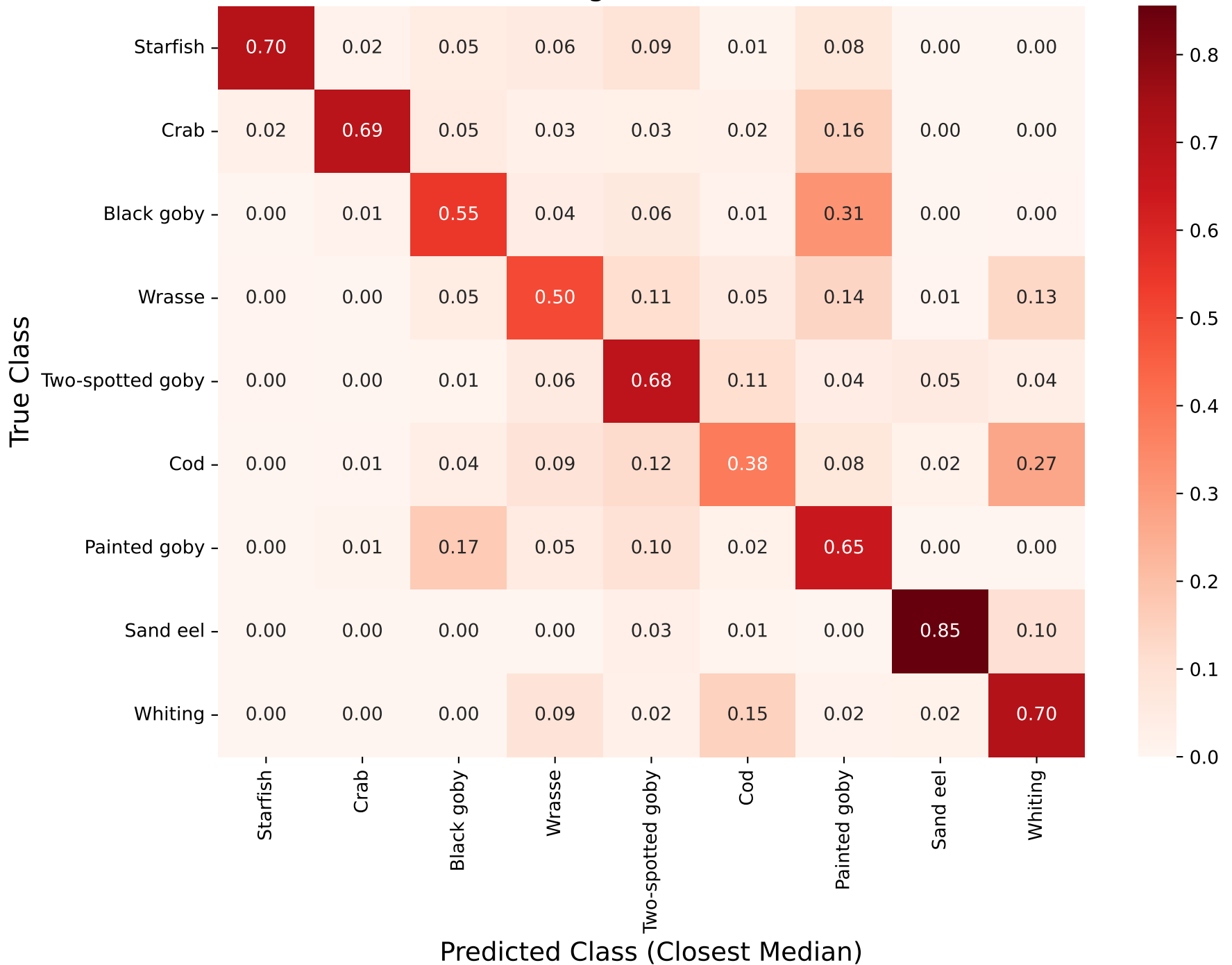
Euclidean Classification Accuracy (Row Normalized) Before Filtering (Euclidean Distance)
