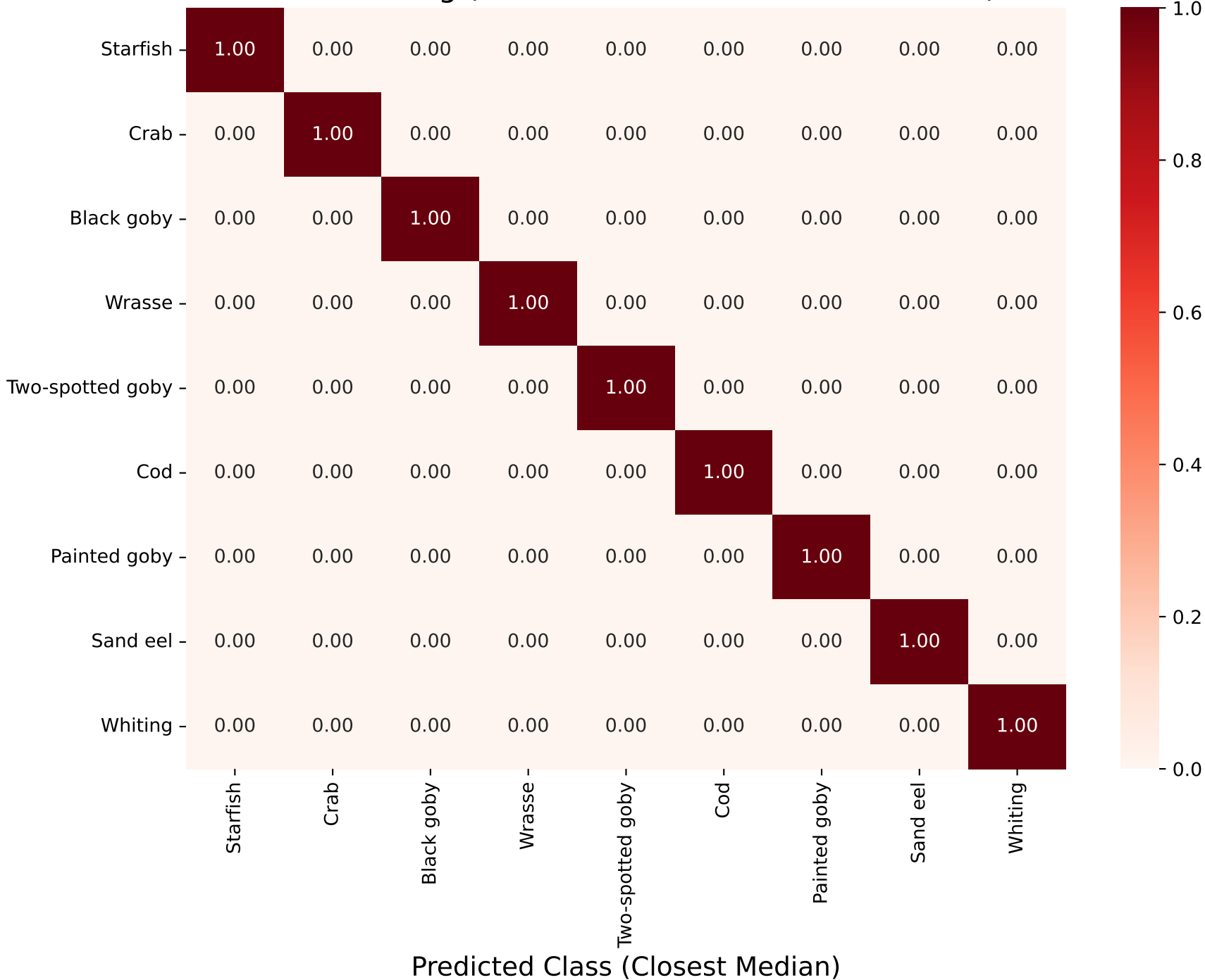
Median Classification Accuracy (Normalized) After Filtering (Classified with ORIGINAL Medians)
