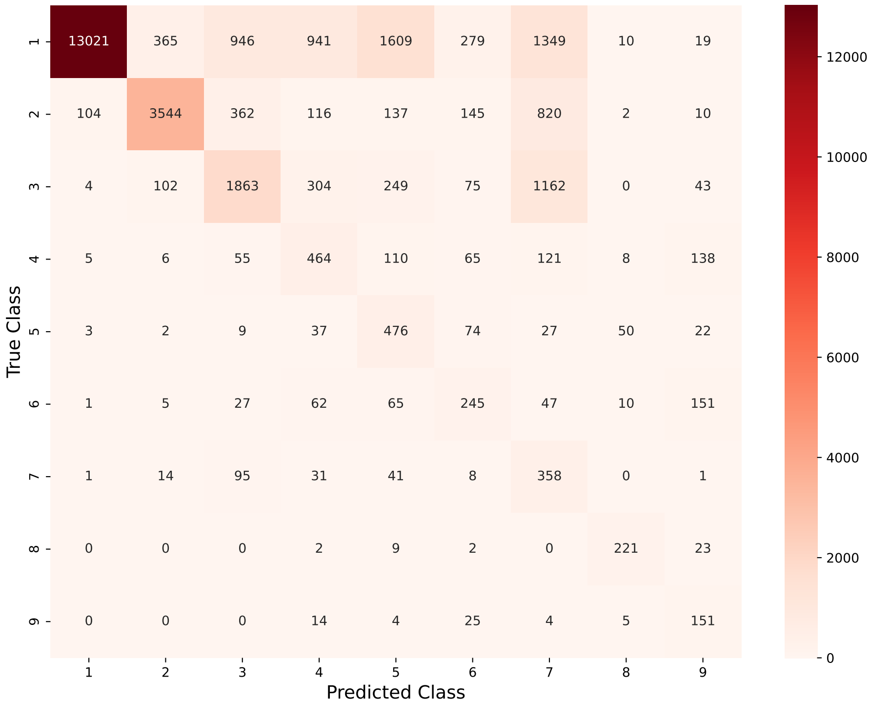
Confusion Matrix — Raw Counts
