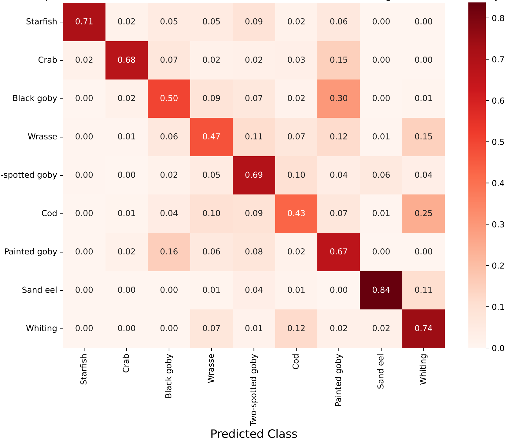
Heat map (row normalised) of DINOv2 normalised embeddings - median analysis
