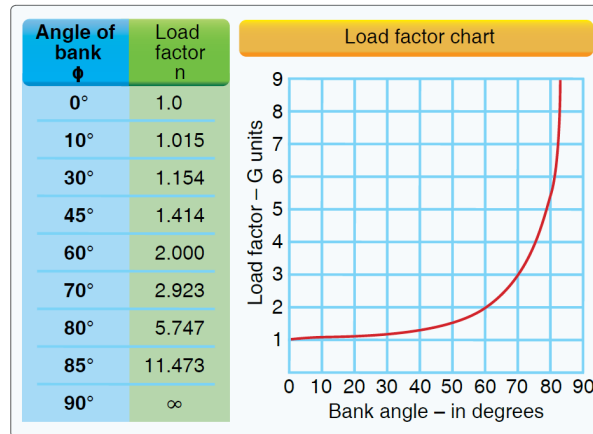
Figure 2. Load Factor Chart.
