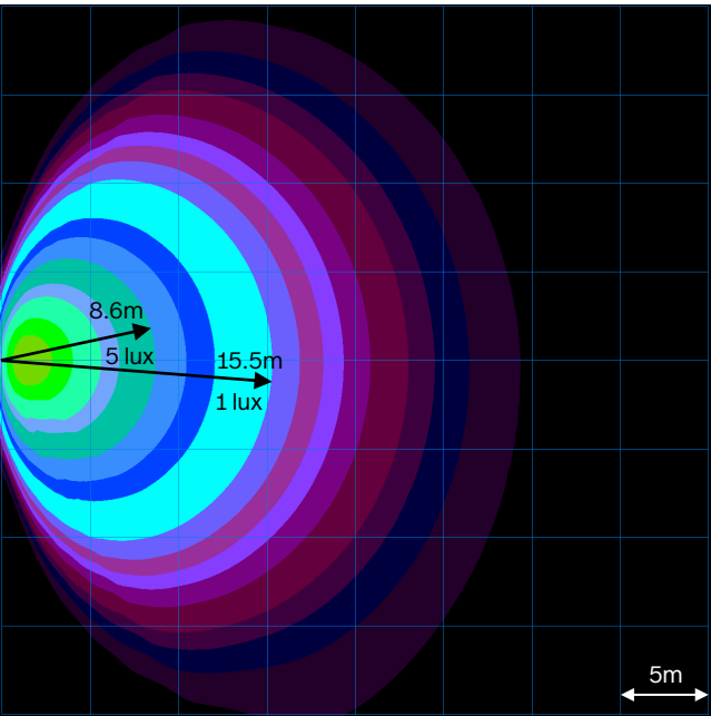
Mounting point 3m high at 20 degrees tilt from vertical
