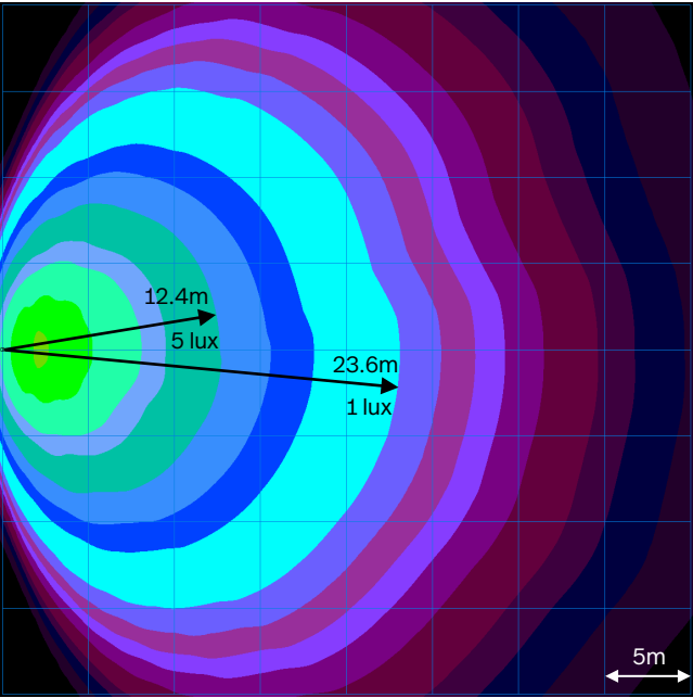
Mounting point 5m high at 20 degrees tilt from vertical
