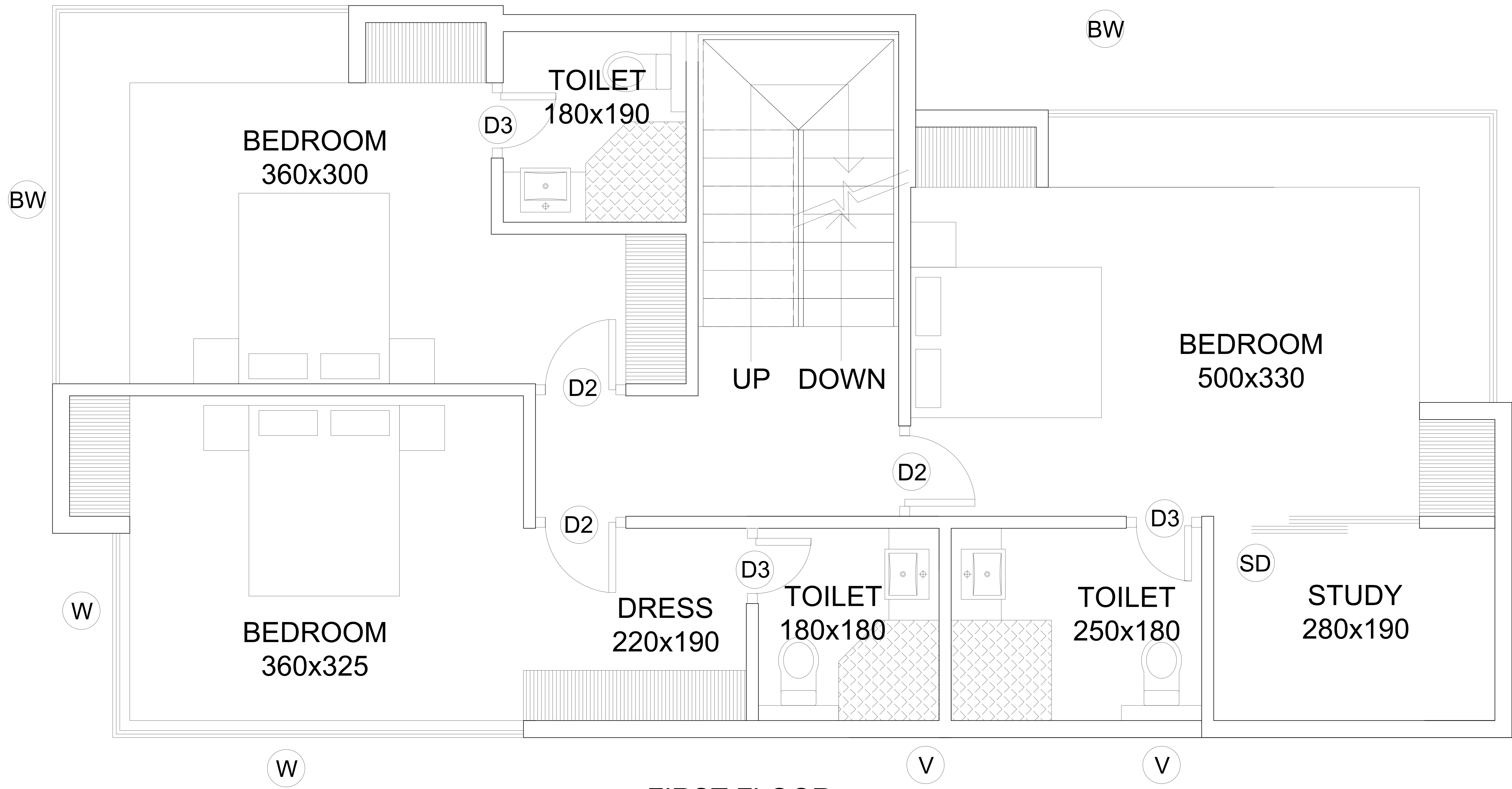
FIRST FLOOR PLINTH AREA - 940 sq. ft. PLINTH AREA - 87.59 sq. m.
