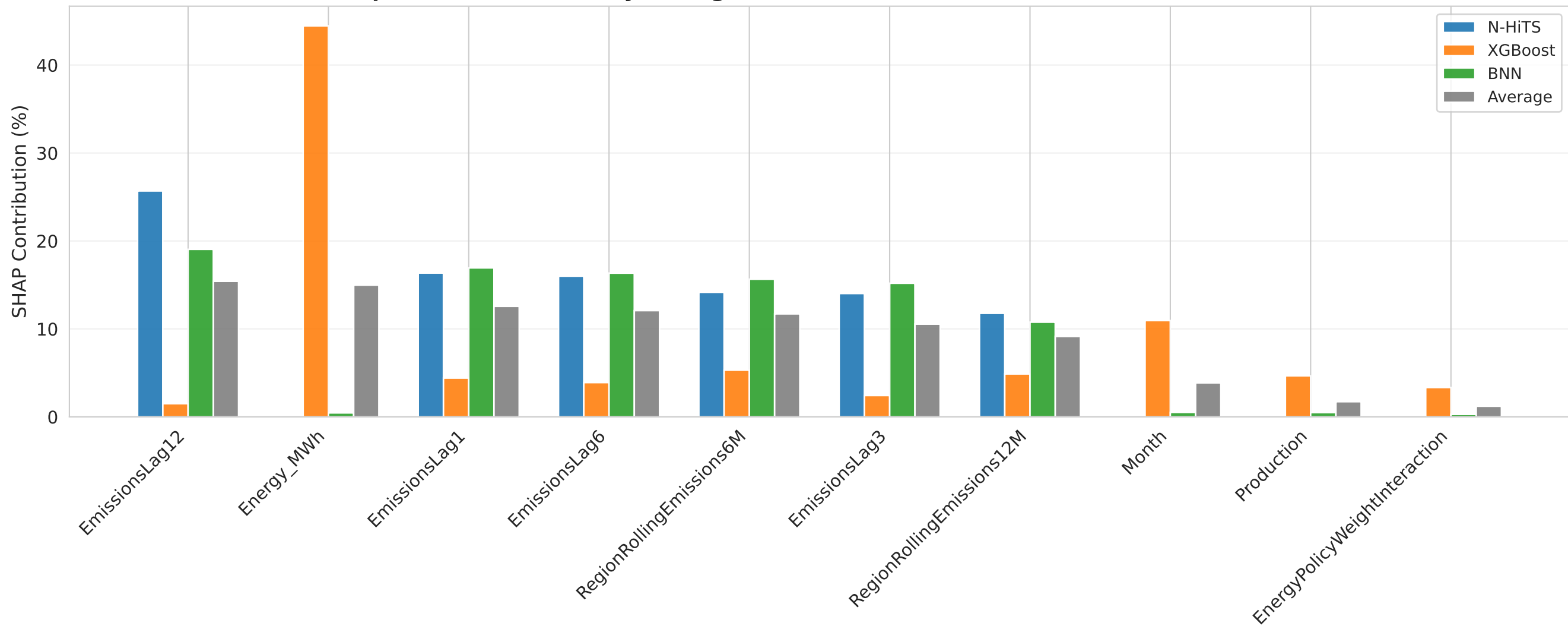
Top 10 SHAP Features by Average Contribution Across N-HiTS, XGBoost, and BNN
