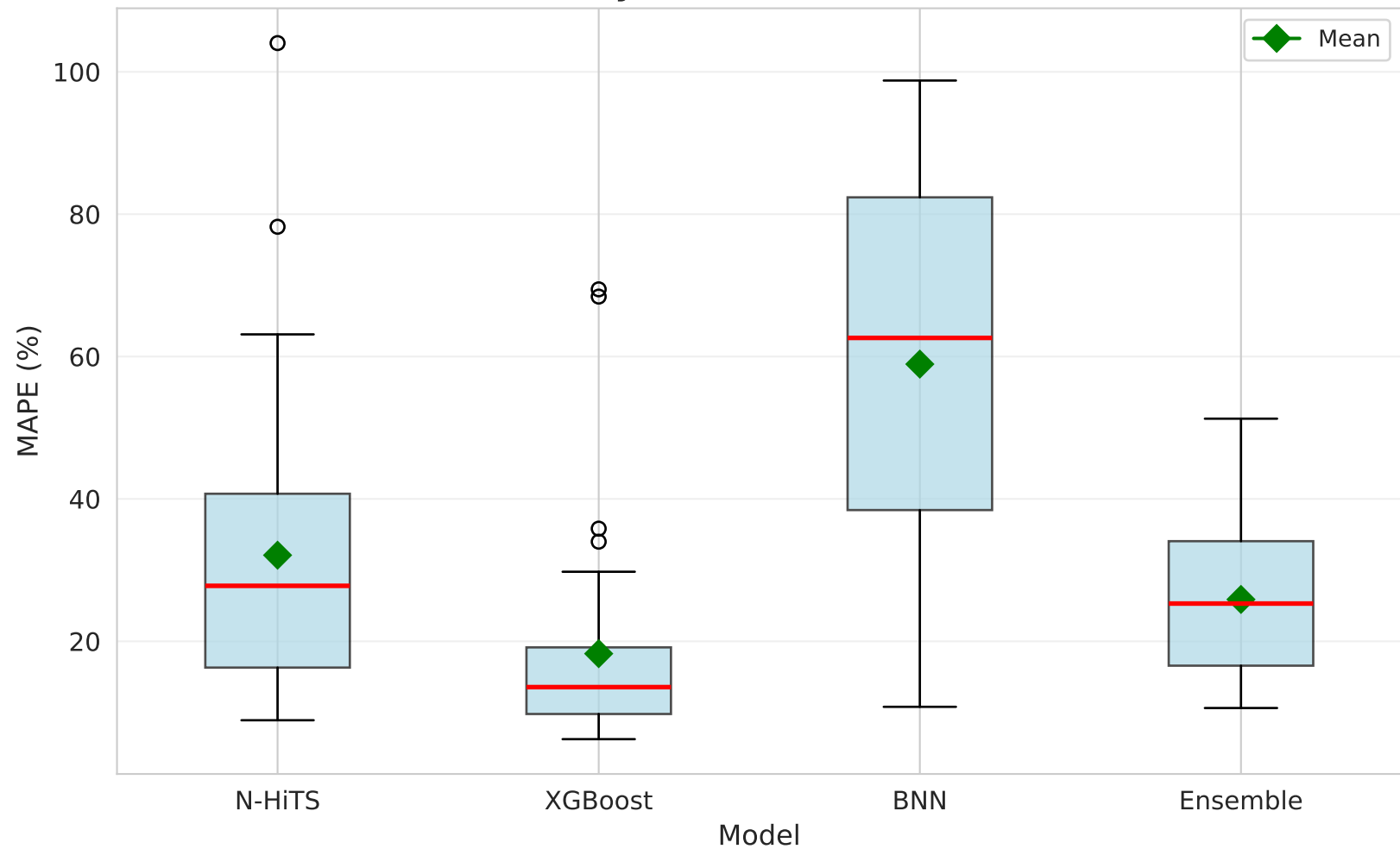
Model Accuracy Distribution Across Facilities
