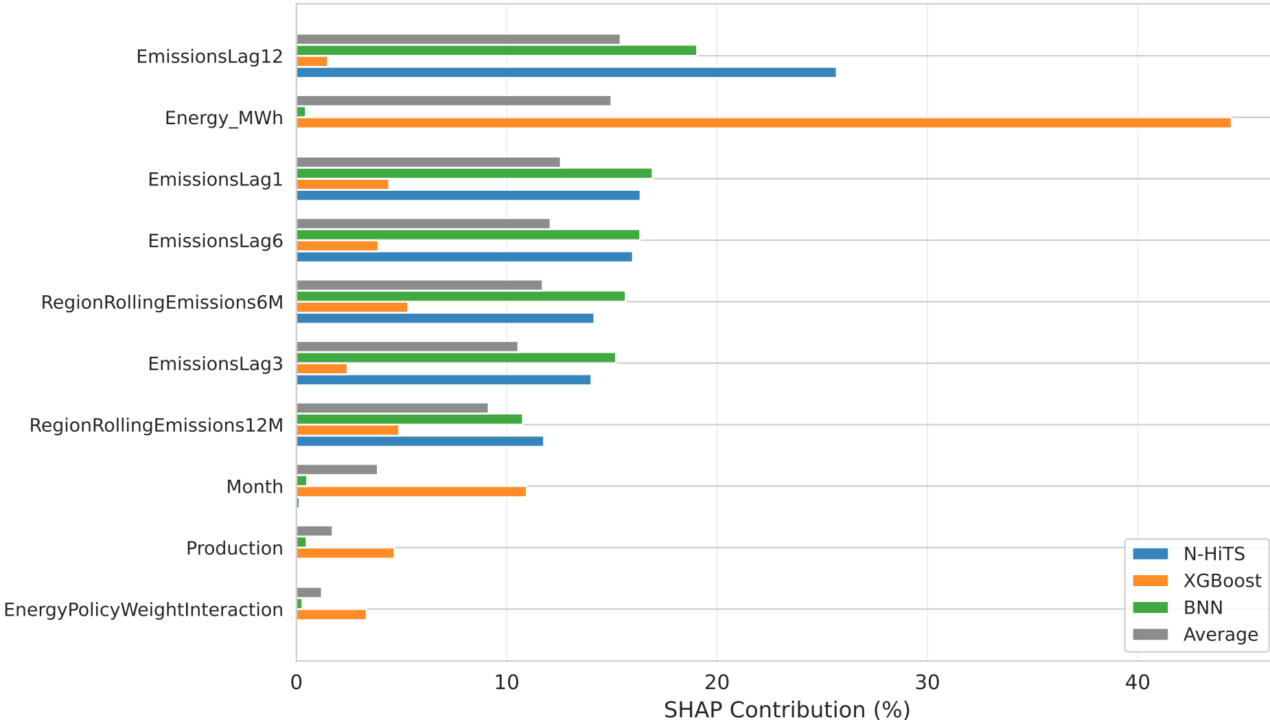
Top 10 SHAP Features by Average Contribution Across N-HiTS, XGBoost, and BNN
