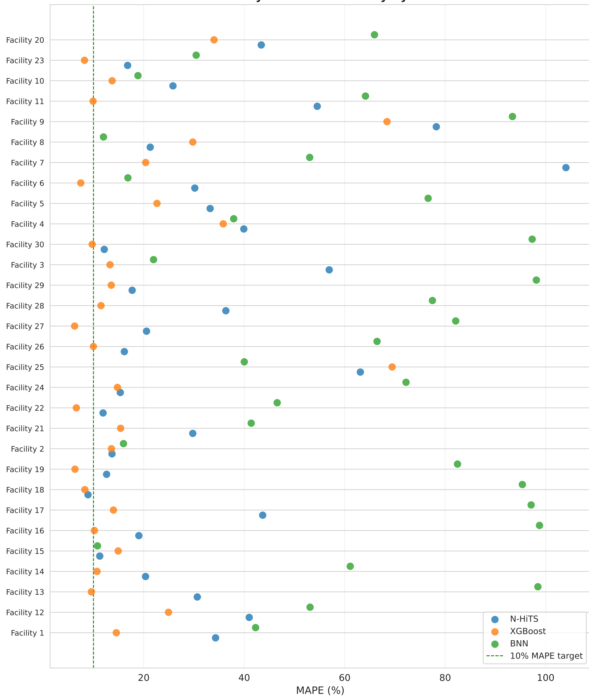
Per-Facility Forecast Accuracy by Model
