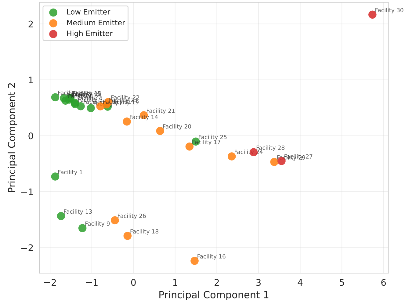
Facility Clusters (K=3) — PCA Projection
