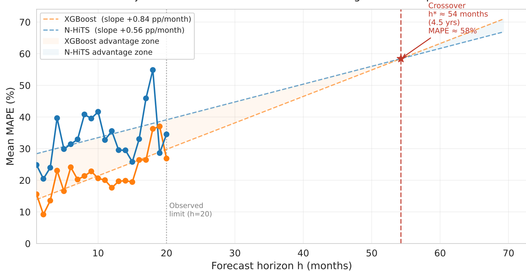
Projected Crossover: XGBoost vs N-HiTS Degradation Slopes
