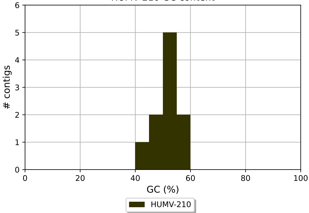
HUMV-210 GC content
