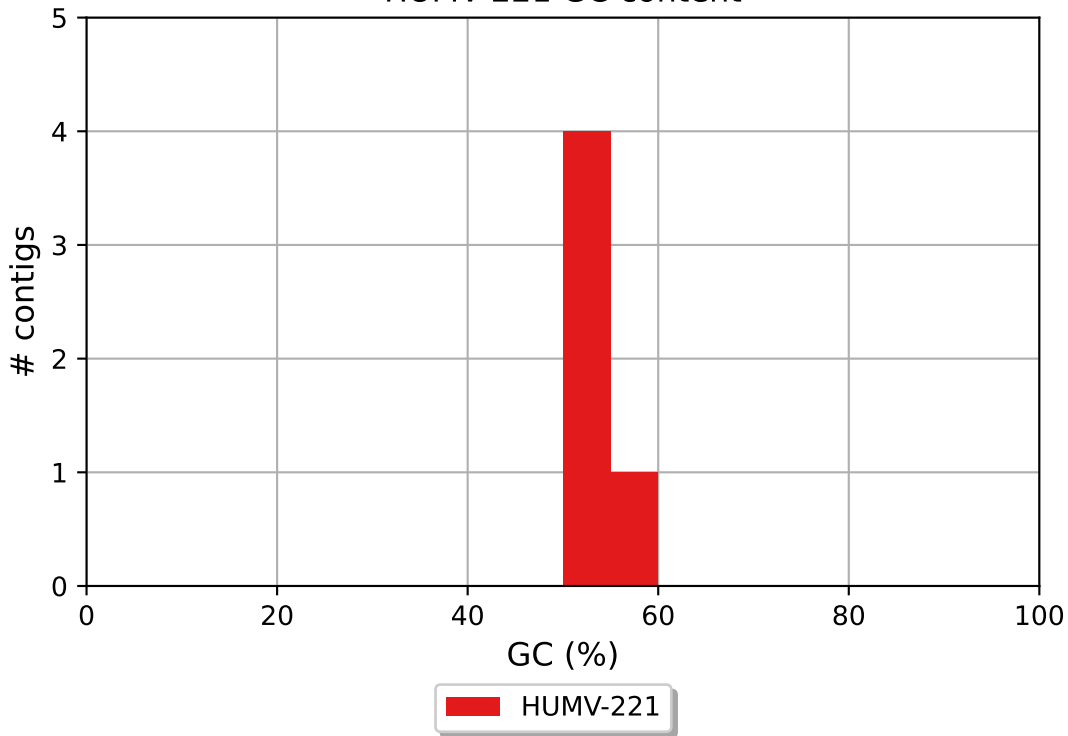
HUMV-221 GC content
