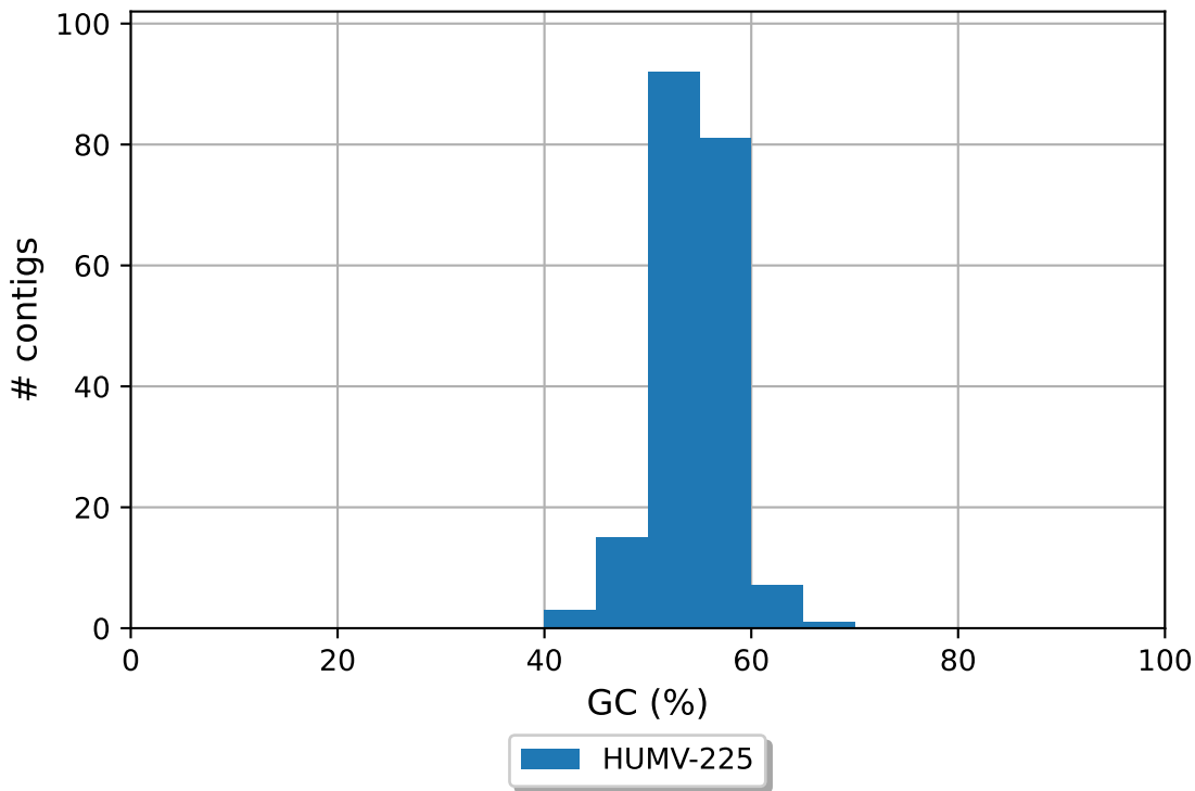
HUMV-225 GC content
