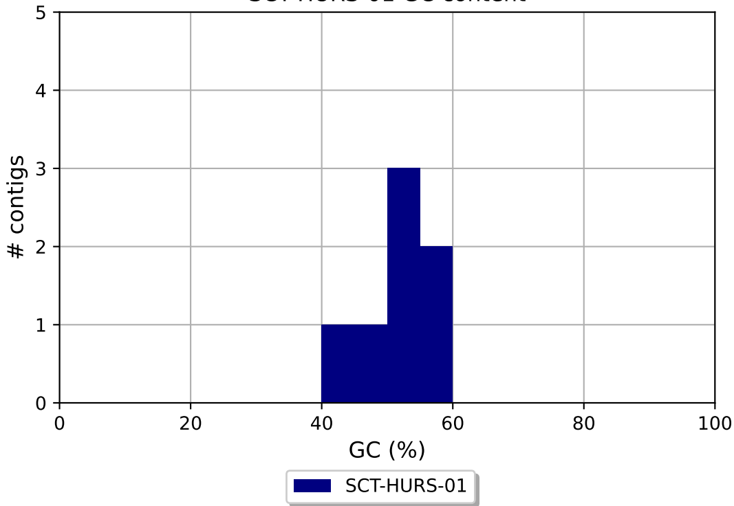
SCT-HURS-01 GC content
