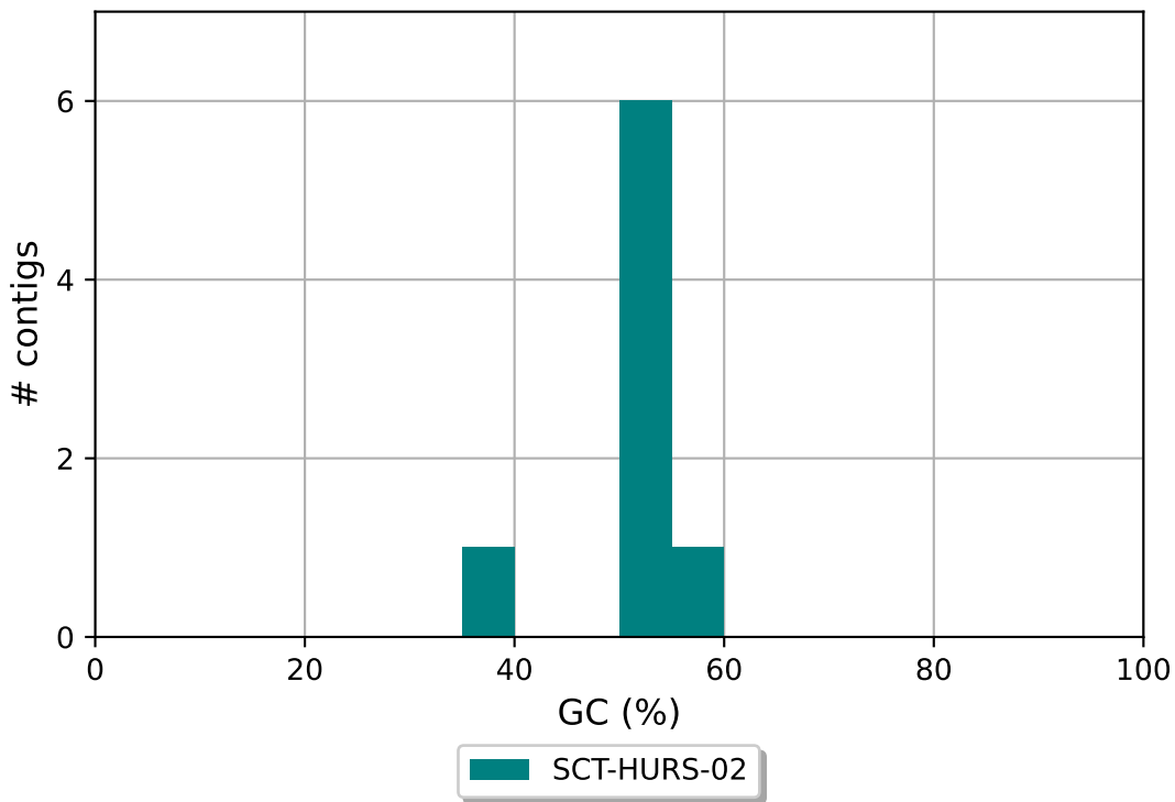
SCT-HURS-02 GC content
