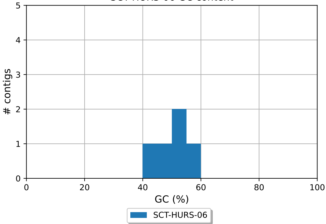
SCT-HURS-06 GC content
