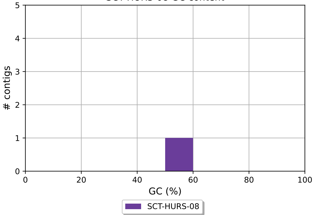
SCT-HURS-08 GC content
