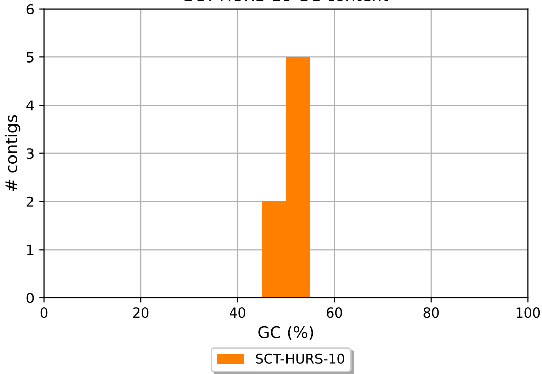
SCT-HURS-10 GC content
