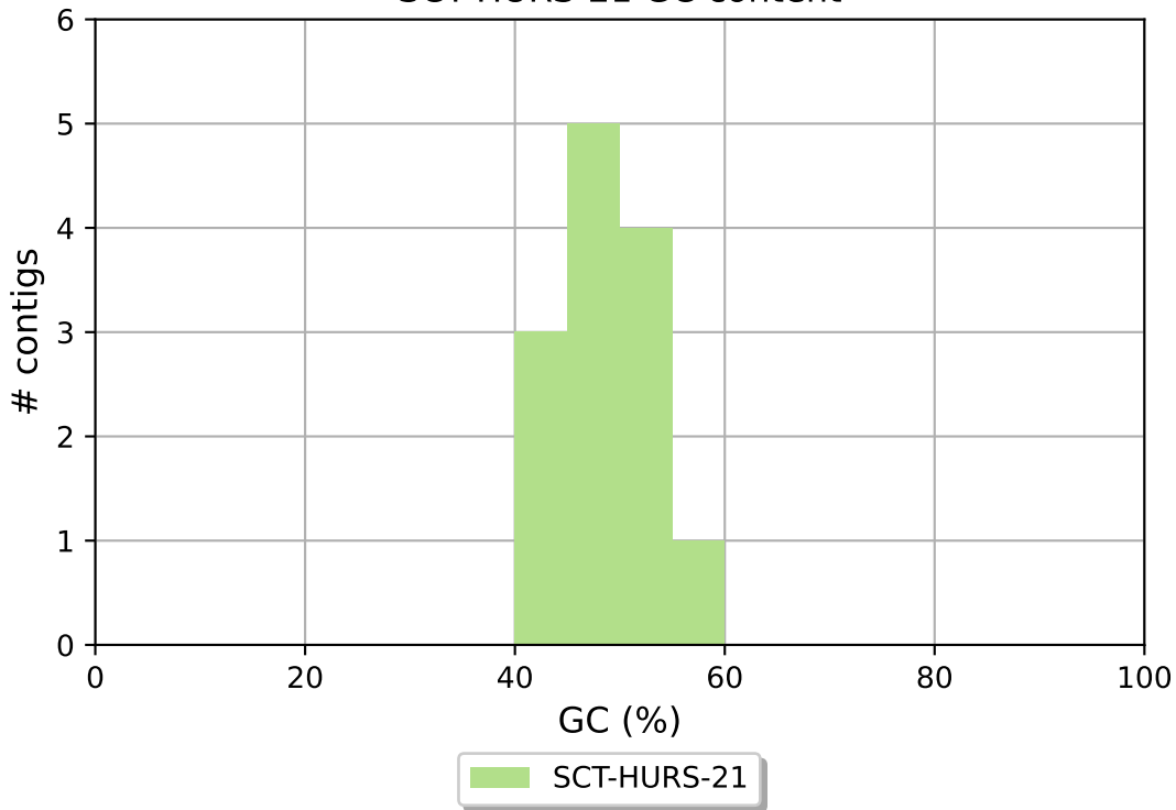
SCT-HURS-21 GC content
