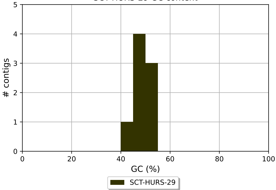
SCT-HURS-29 GC content
