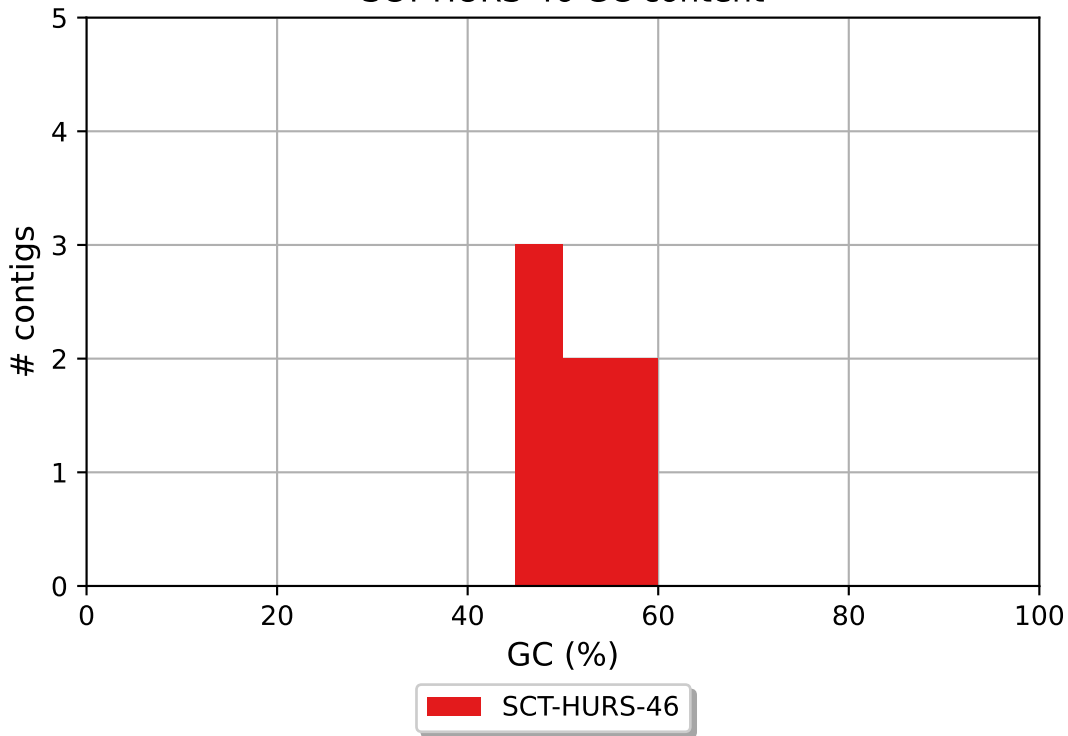
SCT-HURS-46 GC content
