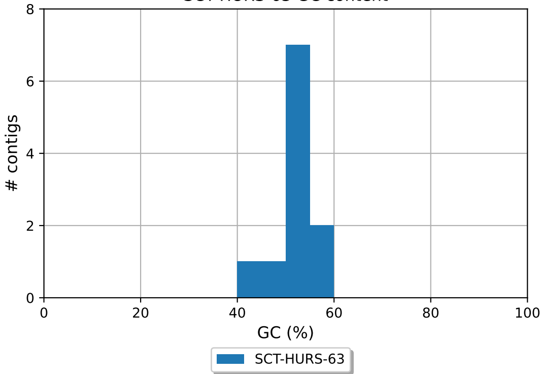
SCT-HURS-63 GC content
