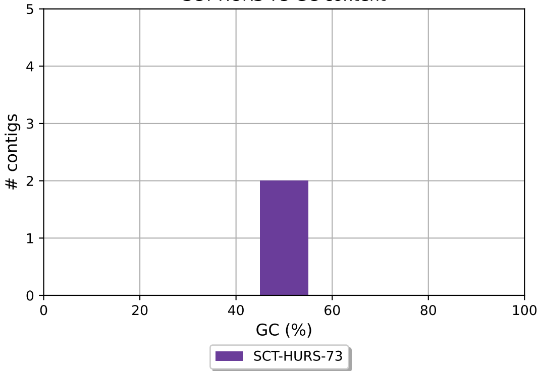
SCT-HURS-73 GC content
