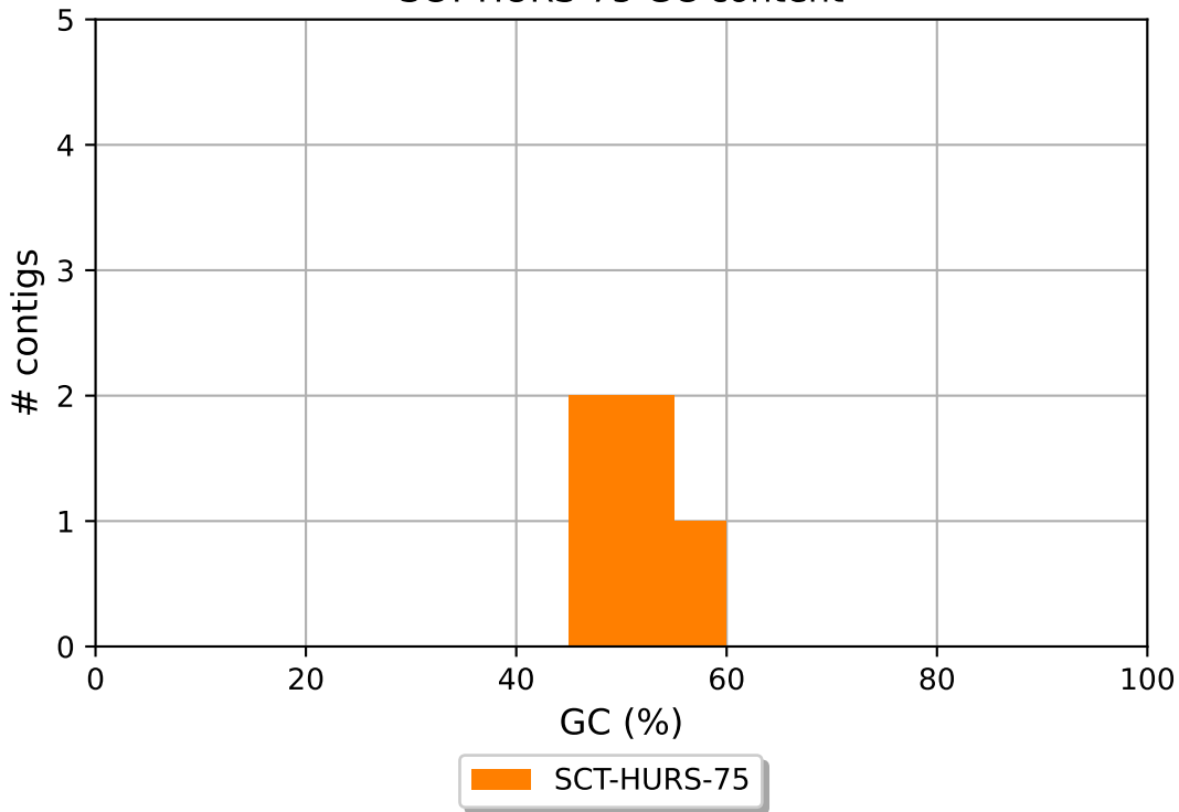
SCT-HURS-75 GC content
