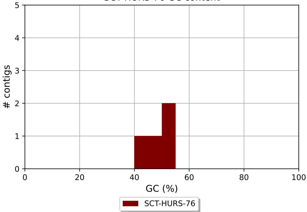
SCT-HURS-76 GC content
