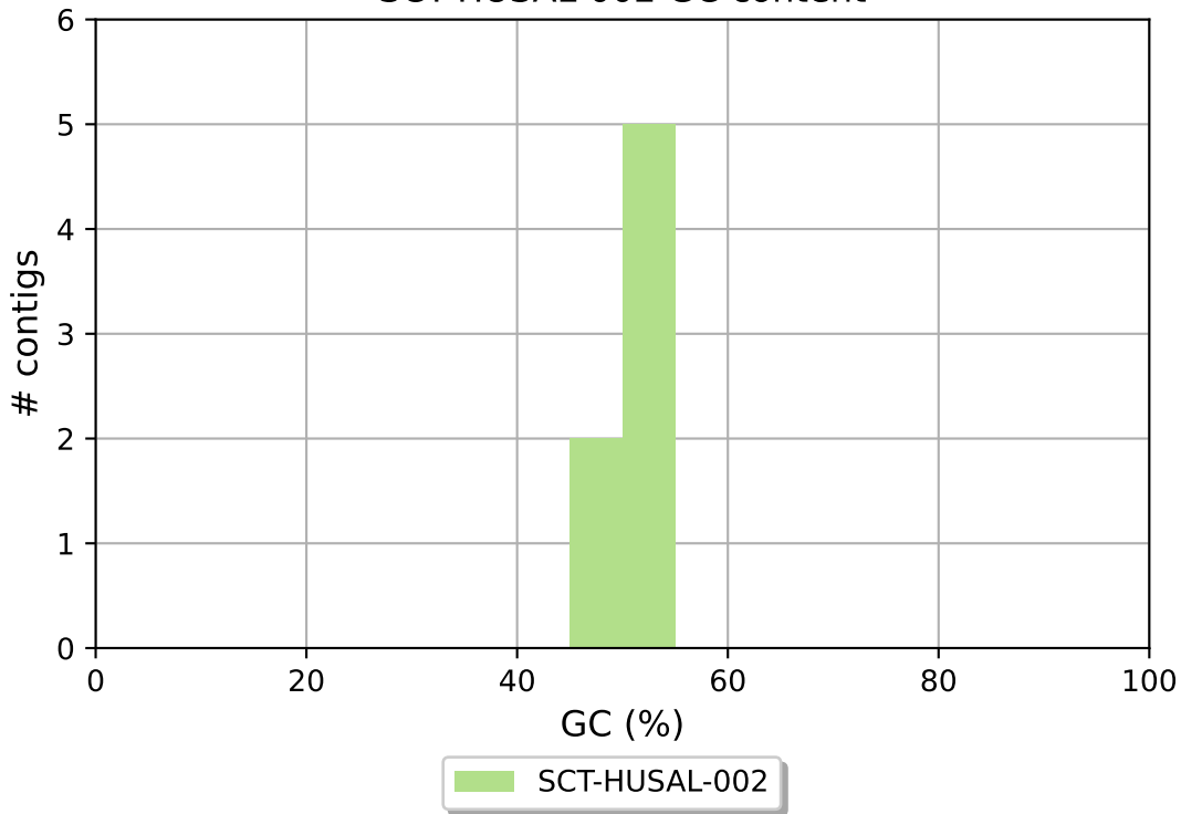
SCT-HUSAL-002 GC content
