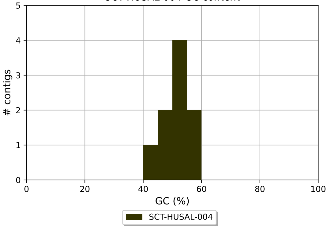
SCT-HUSAL-004 GC content
