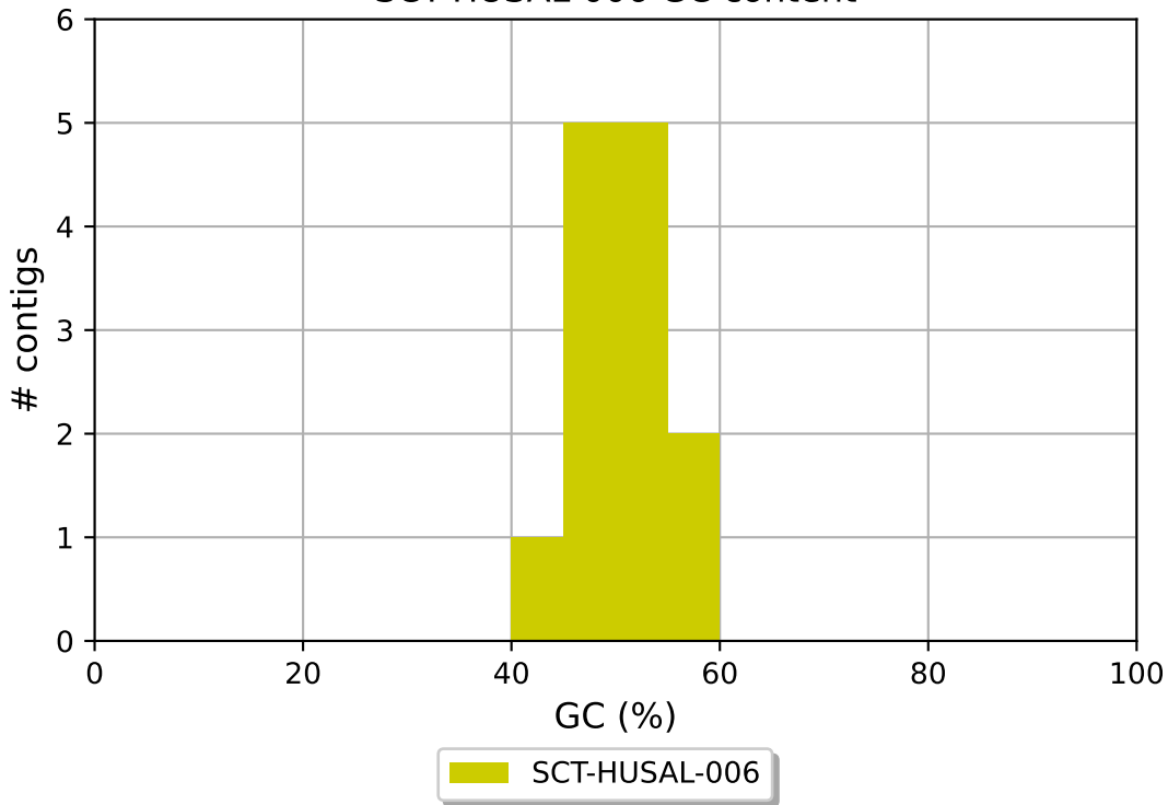
SCT-HUSAL-006 GC content
