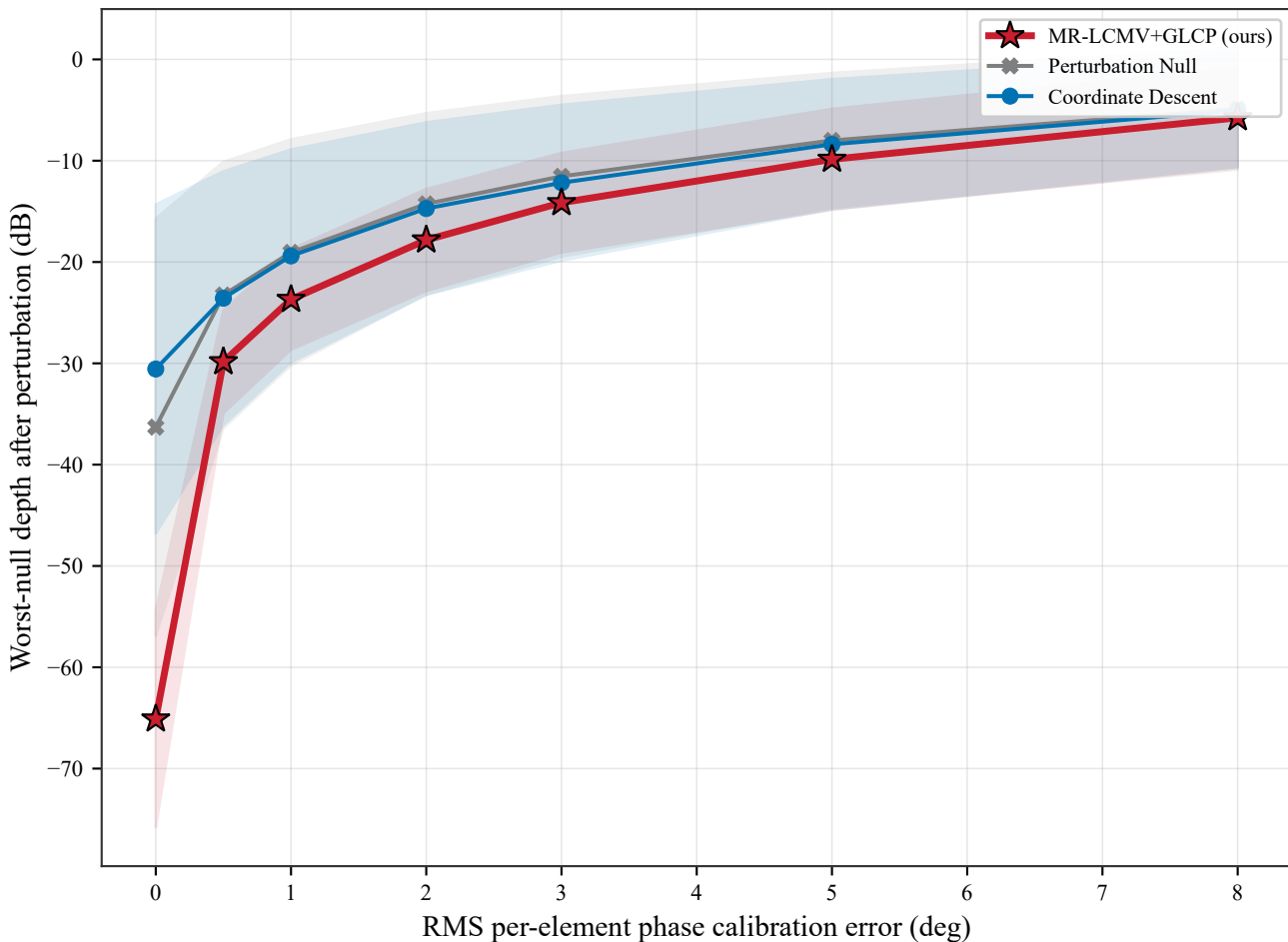
Robustness to calibration error (amplitude error scaled with phase; mean \pm std)
