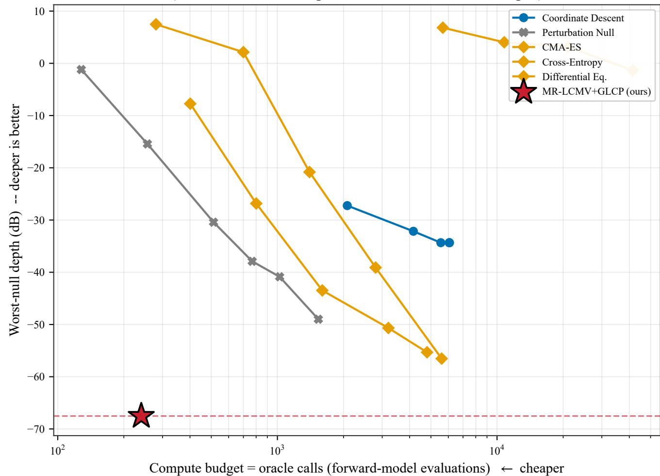
Anytime convergence: null depth vs oracle-call budget (ours = one fixed-cost point; dashed line = its null depth)
