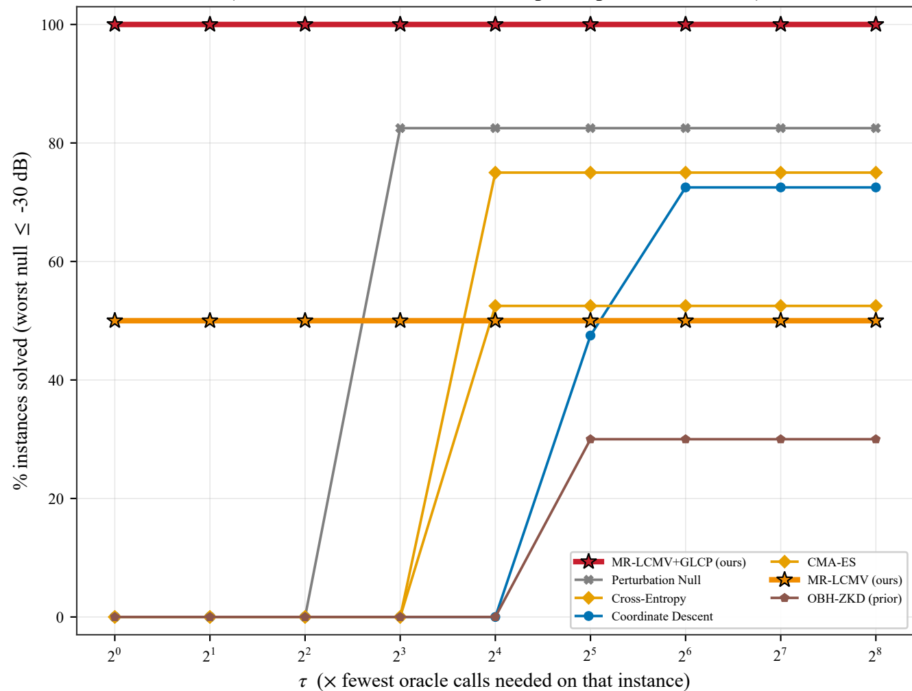
Performance profile keyed on forward-model evaluations (P = 40 instances; left = also cheapest, up = more reliable)
