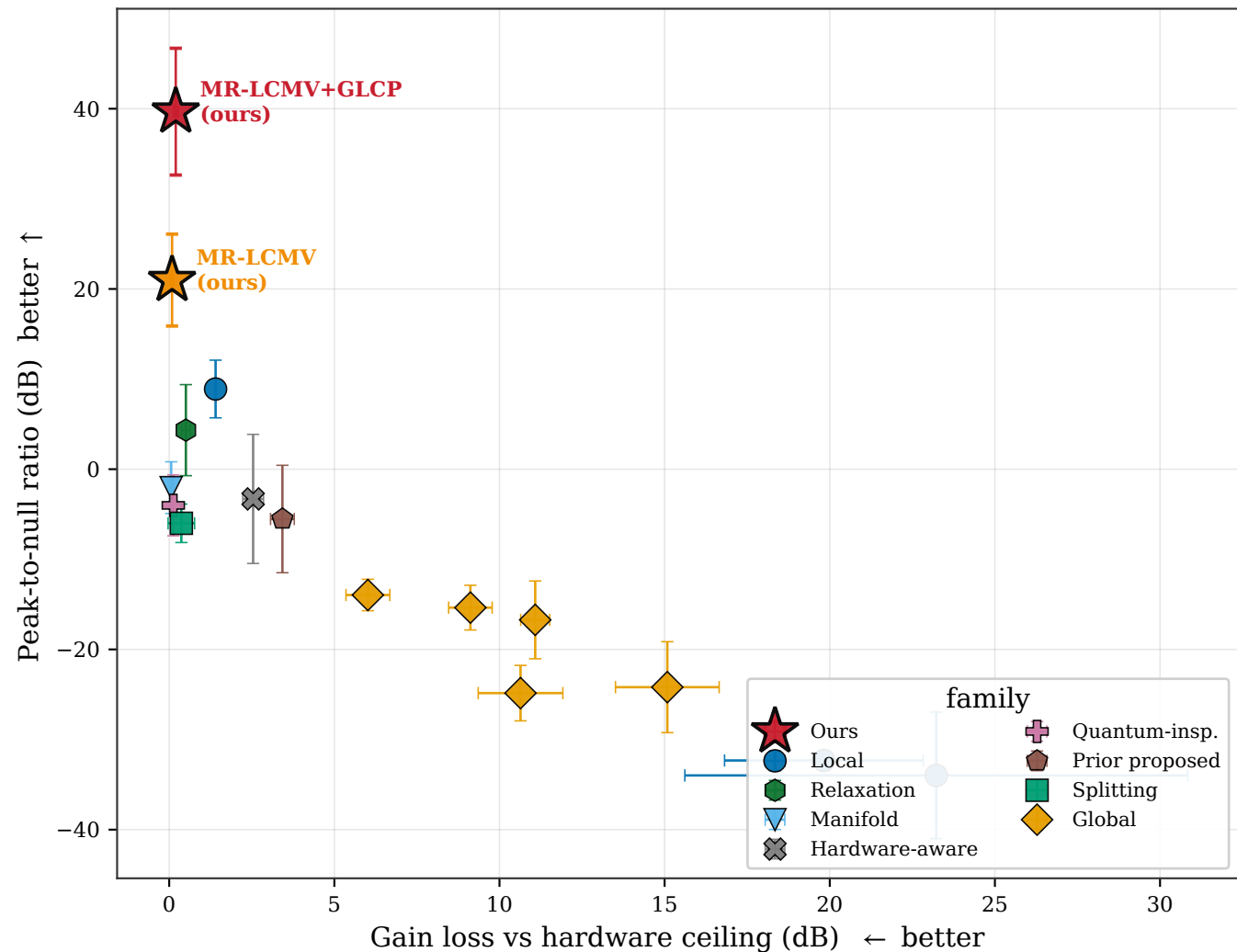
Pareto front: gain retention vs nulling (mean \pm std over random tasks; top-left is best)
