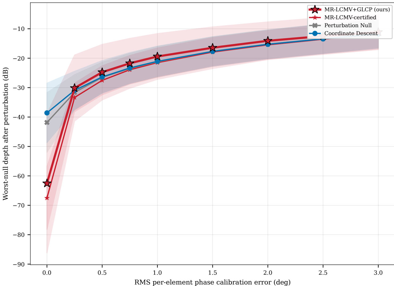
Robustness to calibration error (amplitude error scaled by phase; mean \pm std)
