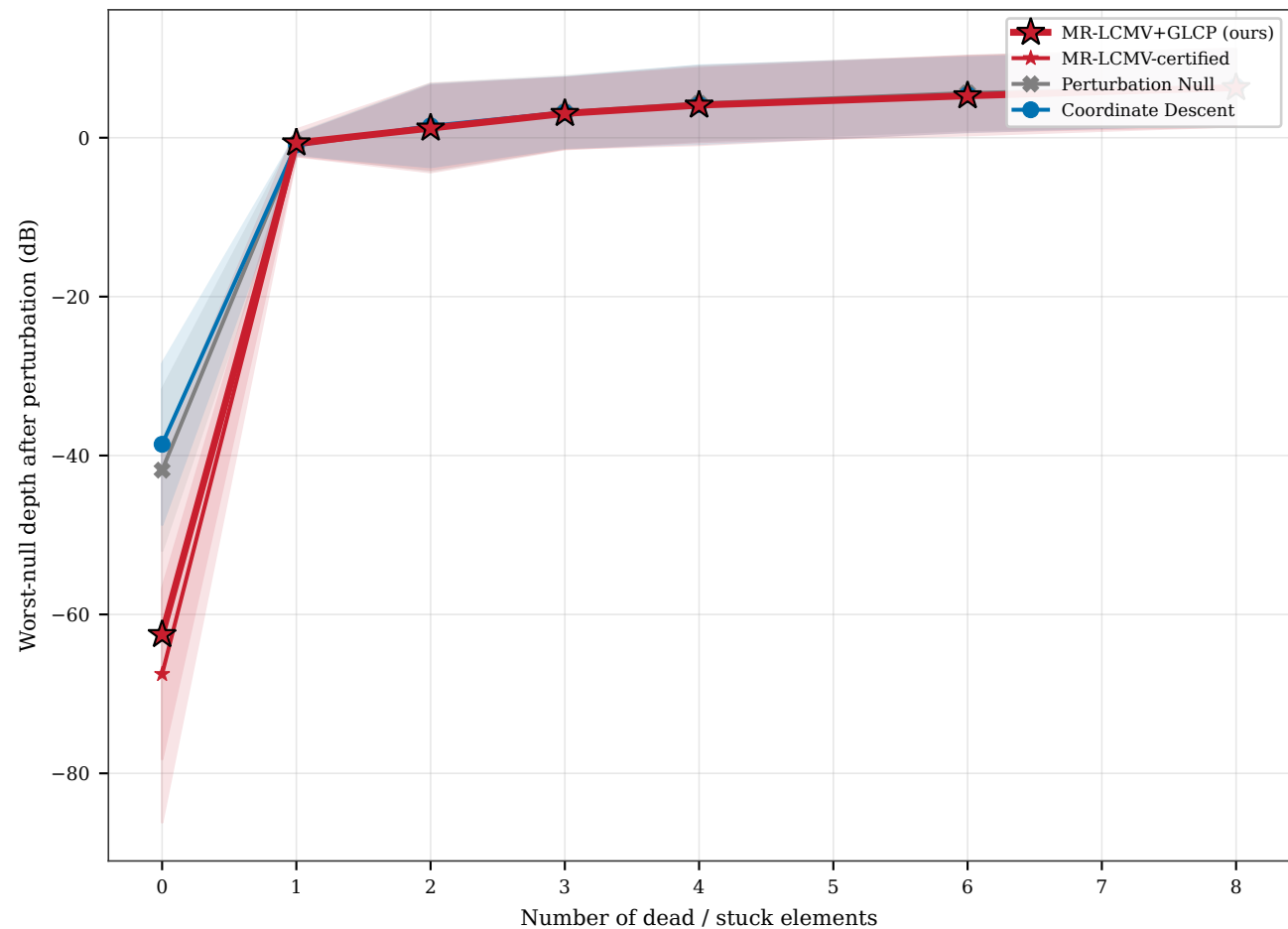
Robustness to element failures (mean \pm std)
