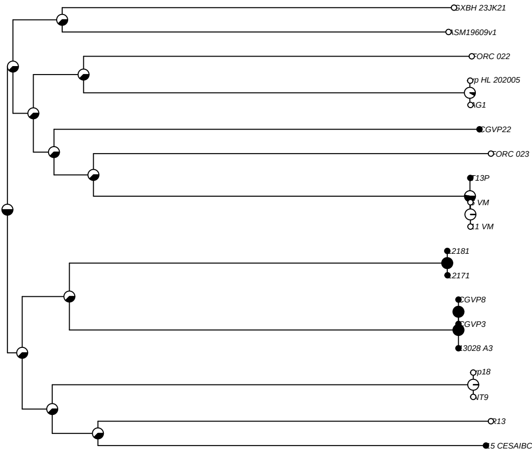
pirA [mean P(present) = 0.435]
