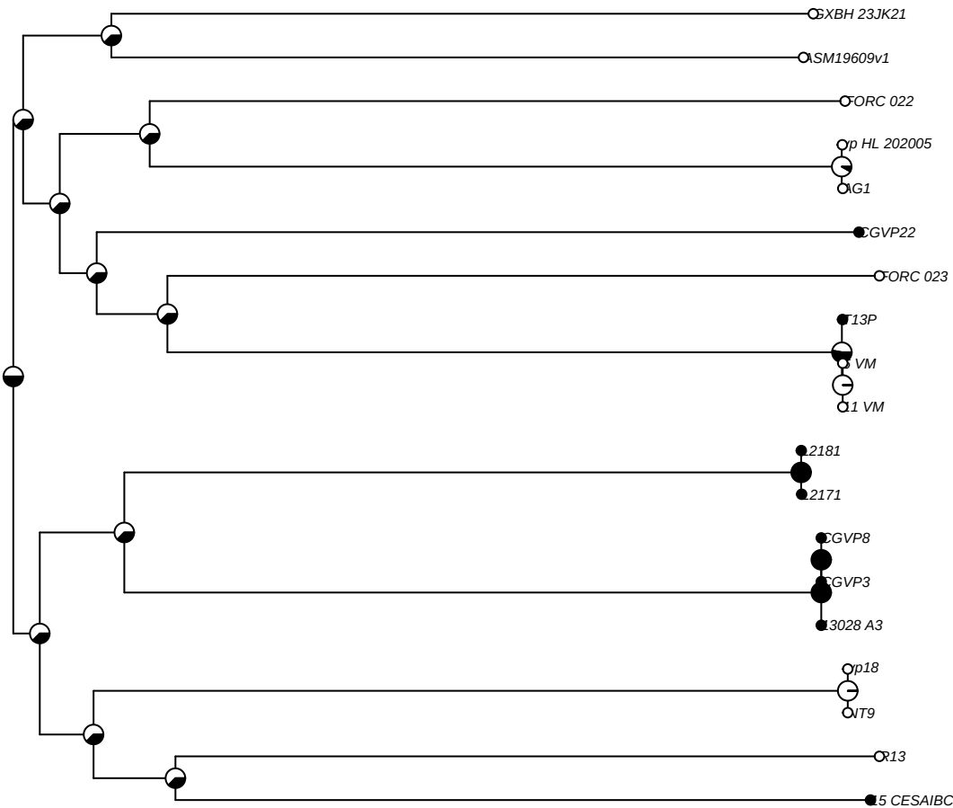
g07720 [mean P(present) = 0.435]
