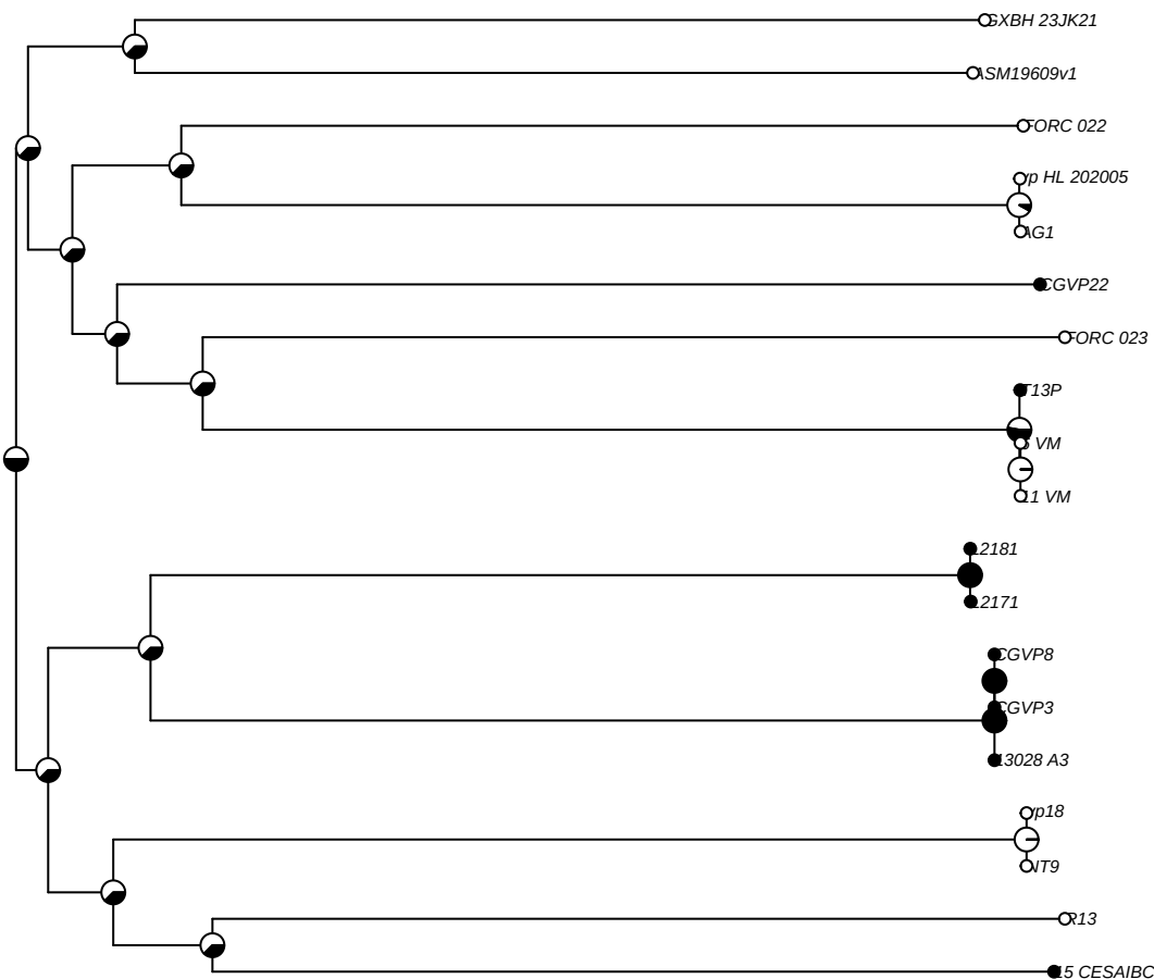
g06662 [mean P(present) = 0.435]
