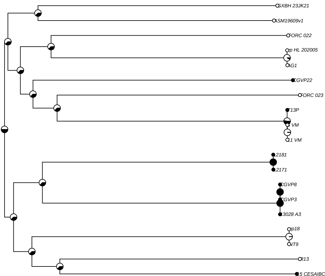
g07221 [mean P(present) = 0.435]
