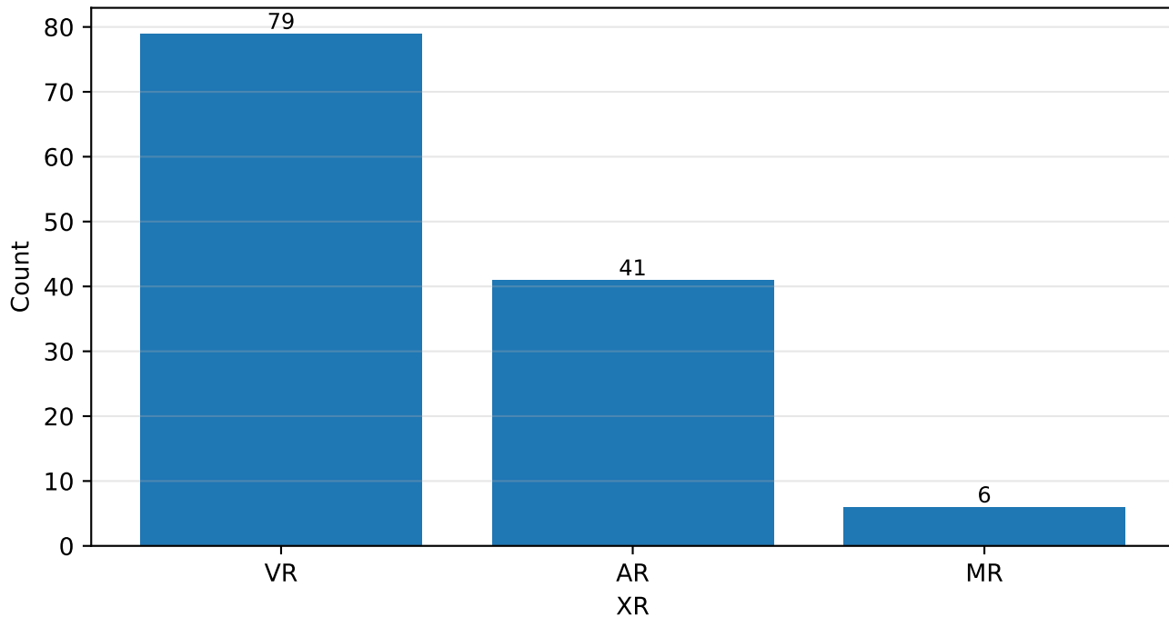
XR distribution
