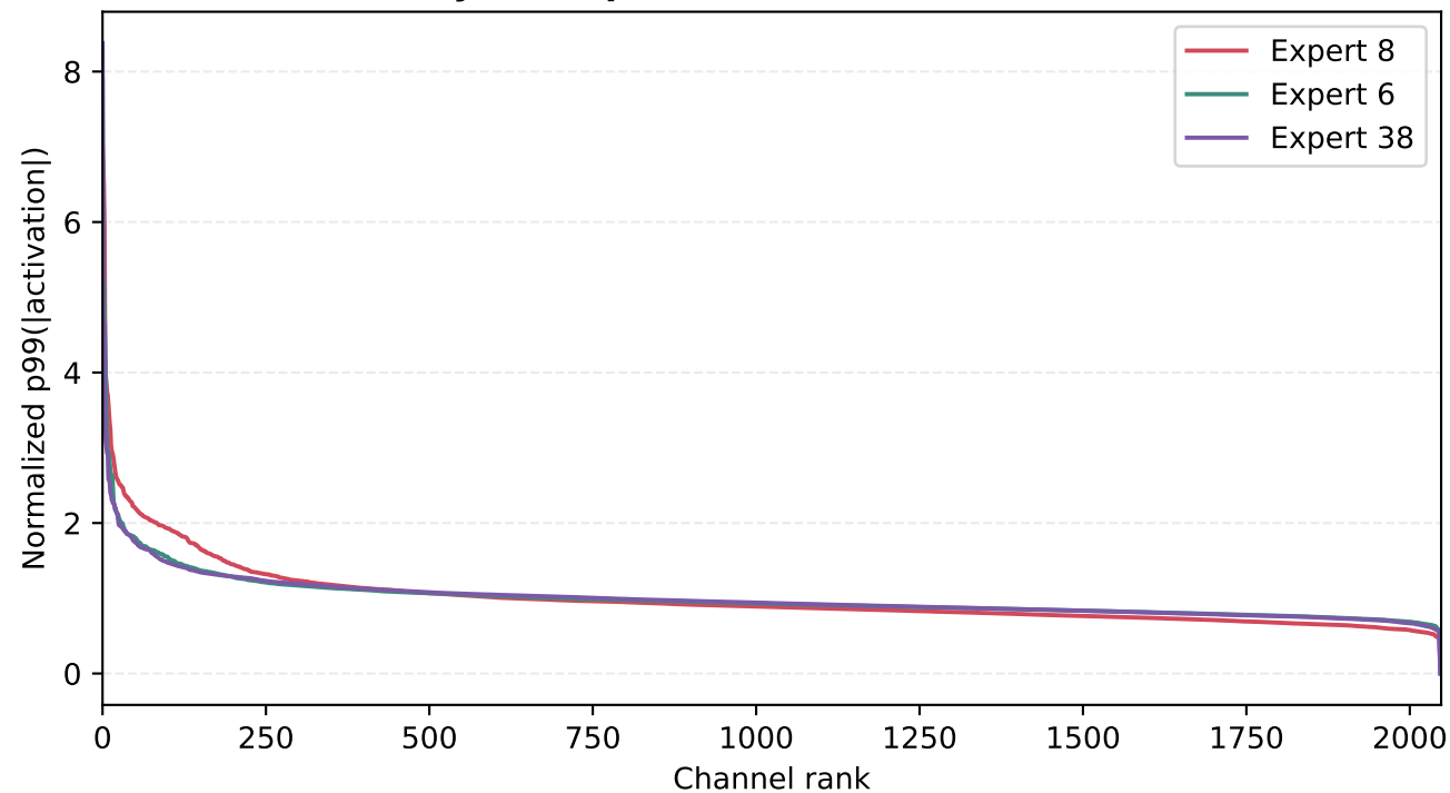
Layer 0 input-channel concentration
