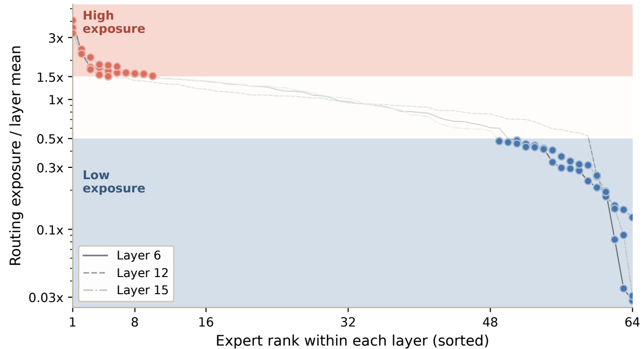
Routing Exposure Long Tail
