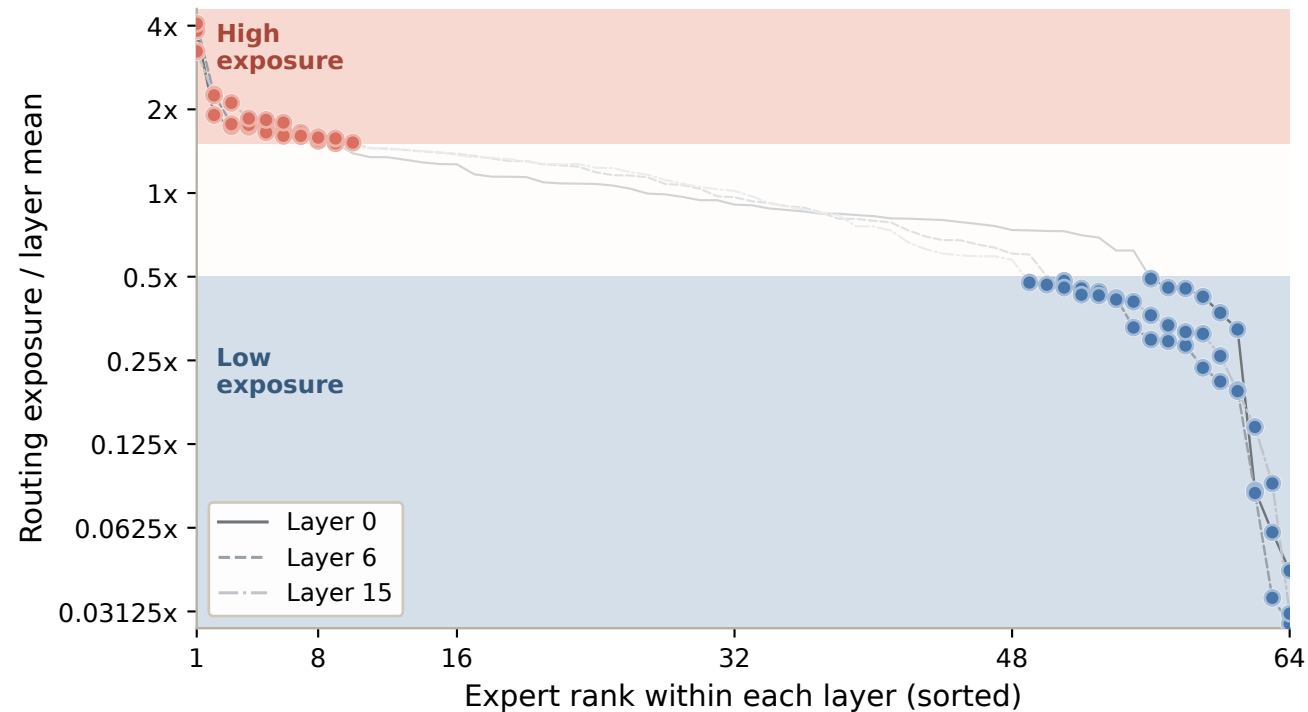
Sorted Routing Exposure Across Experts
