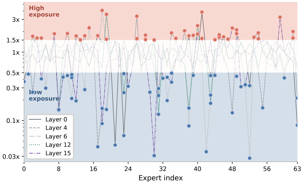
Routing exposure / layer mean
