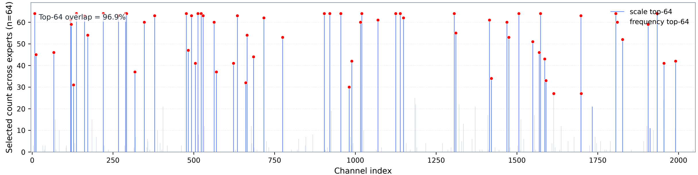
Layer 7 up_proj: top-64 selected-channel frequency
