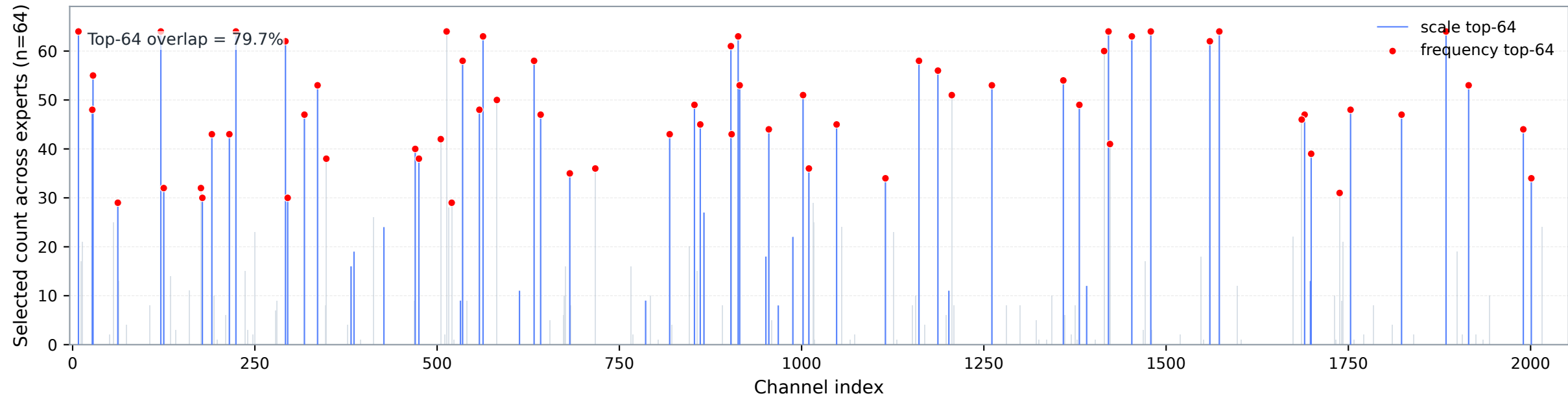
Layer 0 up_proj: top-64 selected-channel frequency
