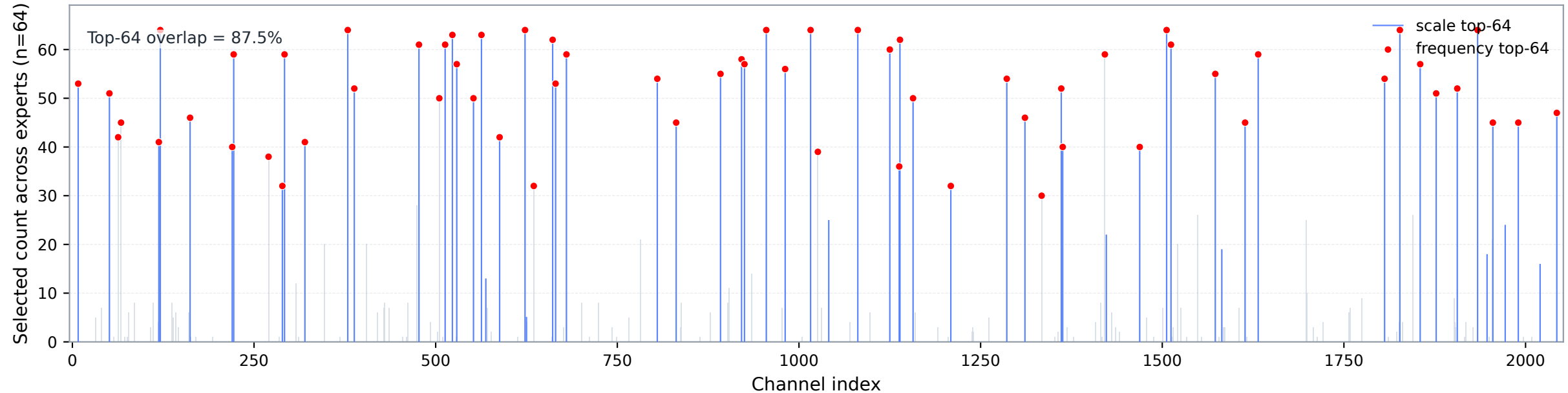
Layer 15 up_proj: top-64 selected-channel frequency
