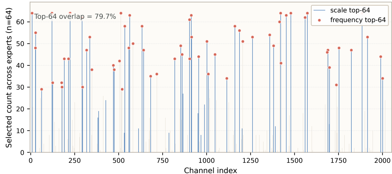
Layer 0 up_proj: top-64 selected-channel frequency
